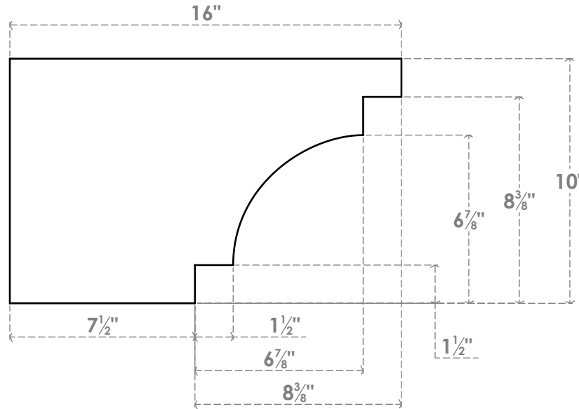
SIDE PROFILE
